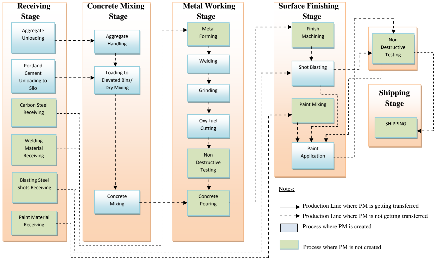
Figure 1: Process Flow Diagram – Particulate Matter through all the stages
